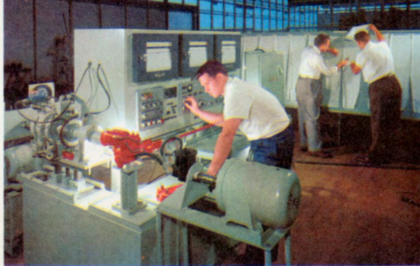
An automatic computing and recording efficiency test stand for steering gear assemblies.
