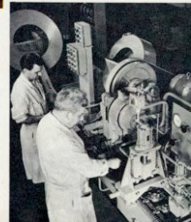
Radiator cap assembly machine designed and built by Manufacturing Development in operation.
