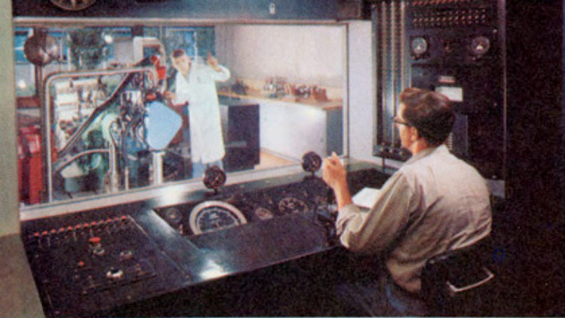
This modern dynamometer installation built to specifications of Research engineers reflects years of experience in engine testing.
