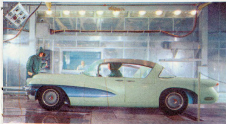
Experience gained in 30 years' operation of automotive cold rooms has resulted in this modern version, where cars can be tested at 90 degrees below zero.
