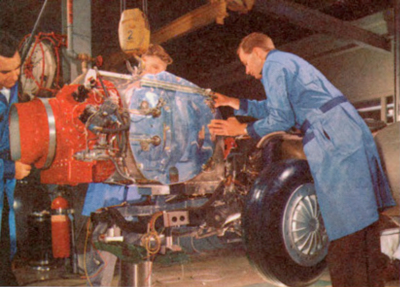
Installing the Whirlfire GT304 gas turbine engine in the Firebird II.
